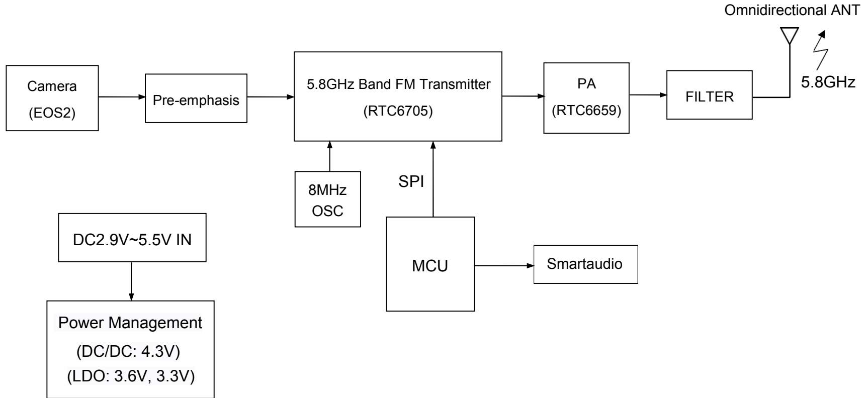
Block Diagram
